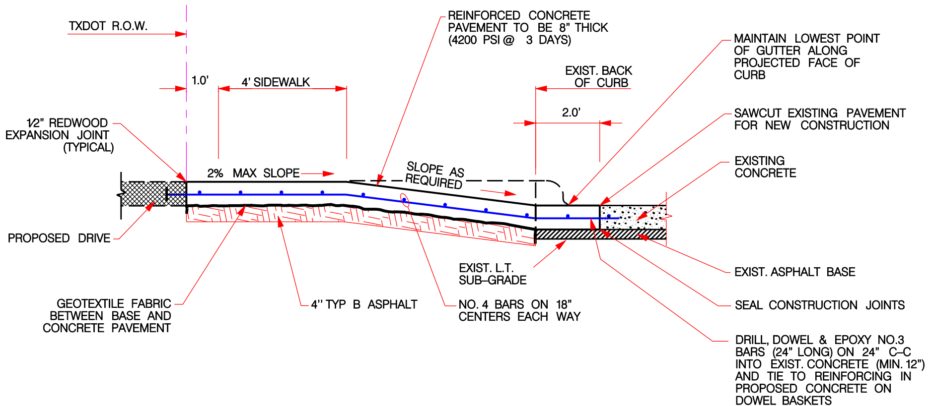
Section View
