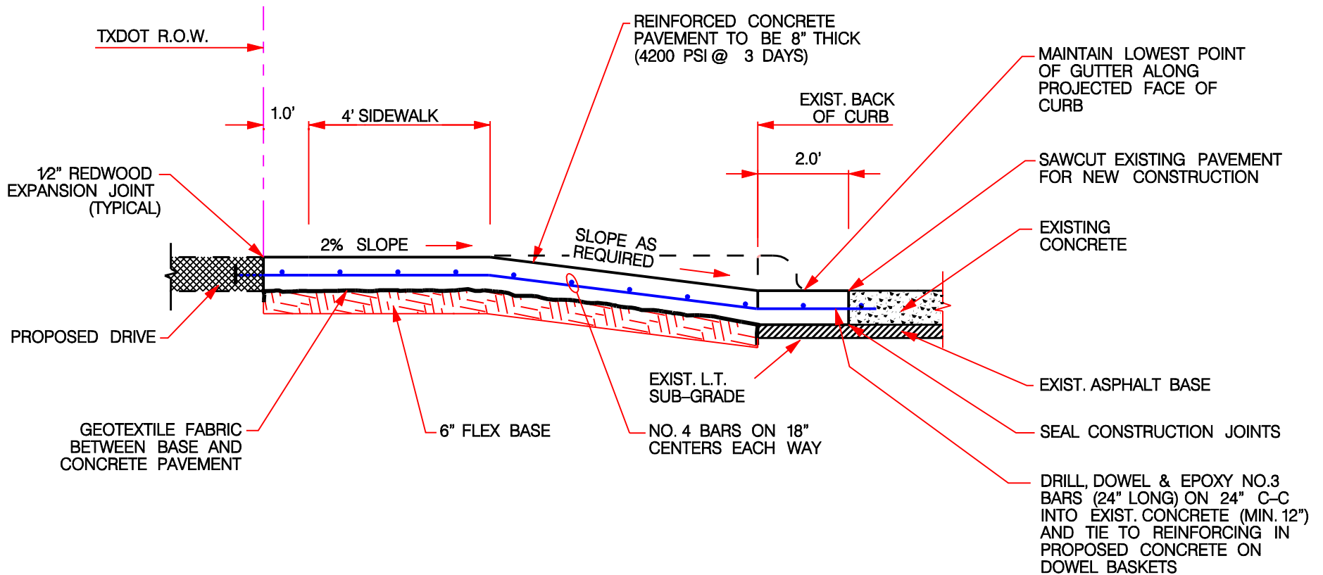
Section View
